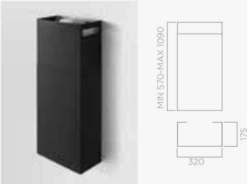
KIT CAMINO NERO BLACK CHIMNEY KIT
